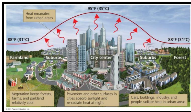
Urban Heat Island Effect
